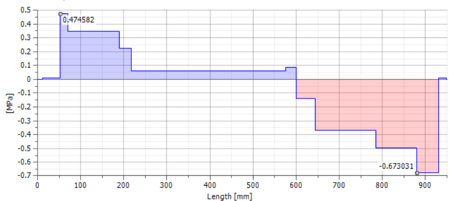
Torsional Stress
