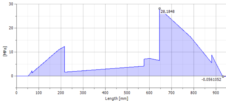
Shear Stress
