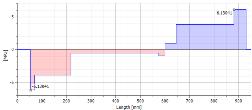
Tension Stress
